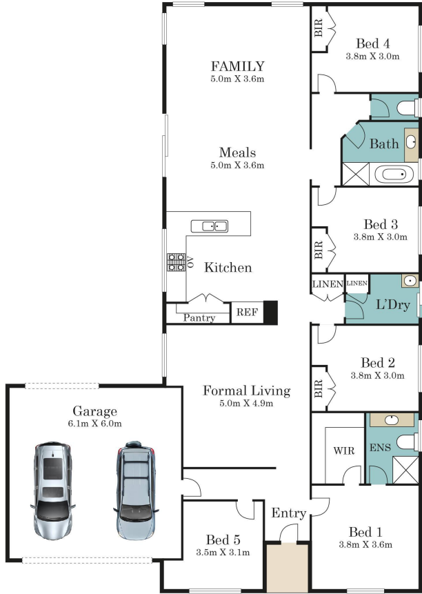
Floor Plan
