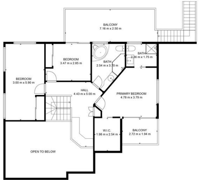
FLOOR 2
