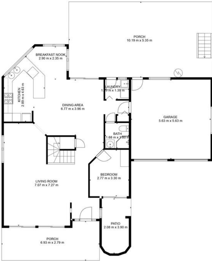
FLOOR 1
