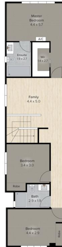
Upper Floor
