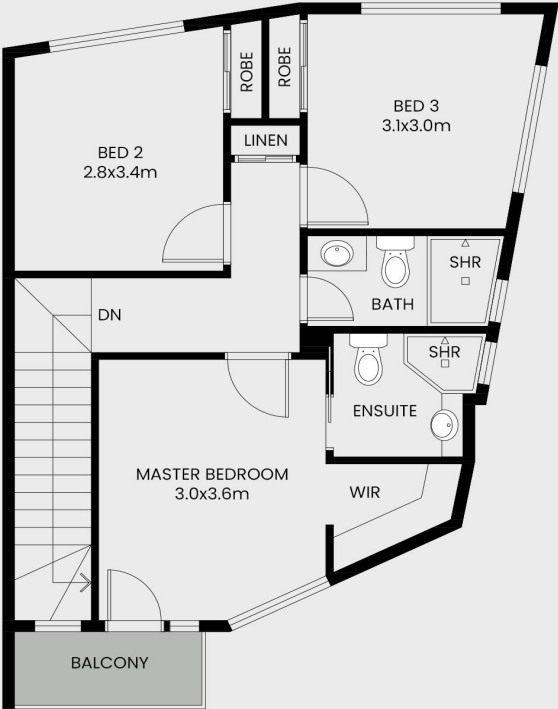
FIRST LEVEL
