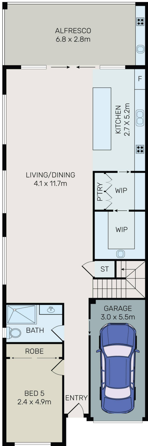
GROUND FLOOR
