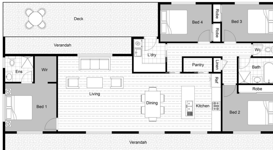
FLOOR PLAN
