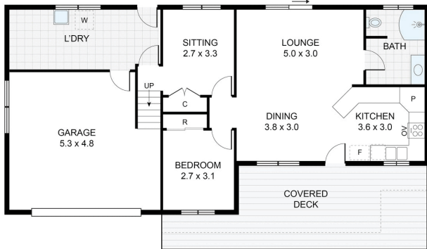
GROUND FLOOR : 120m 2 (INCLUDES GARAGE)
