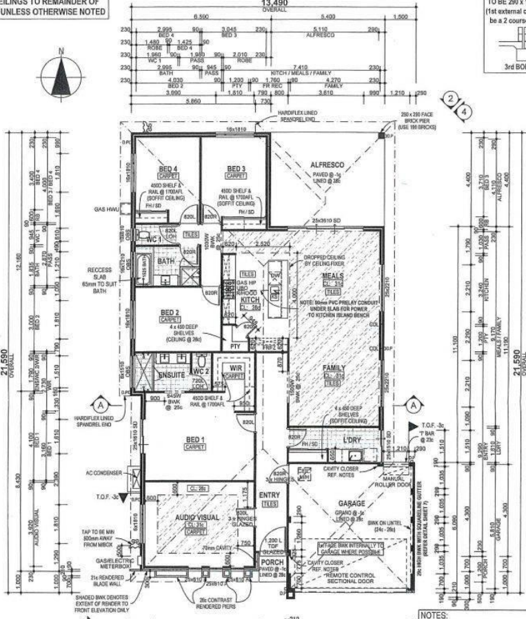
GROUND FLOOR 1:100
