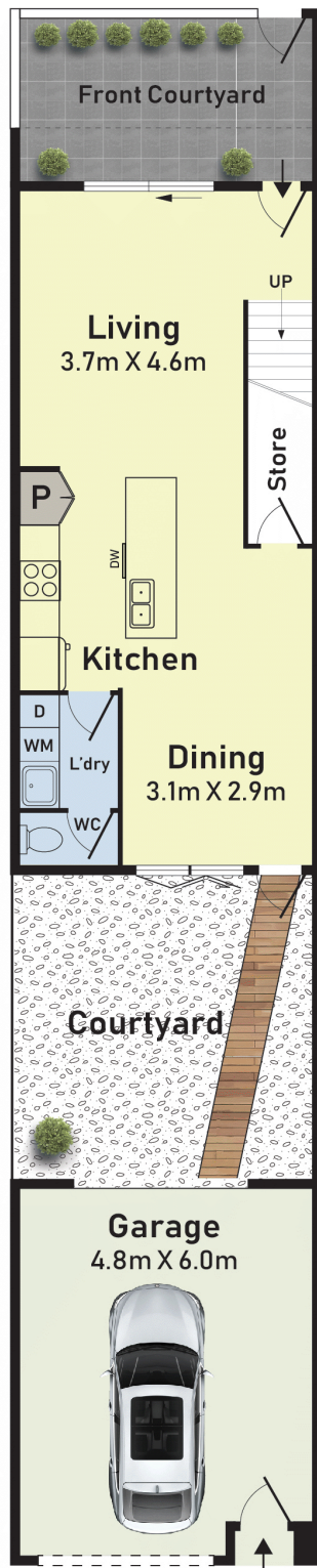
GROUND FLOOR
