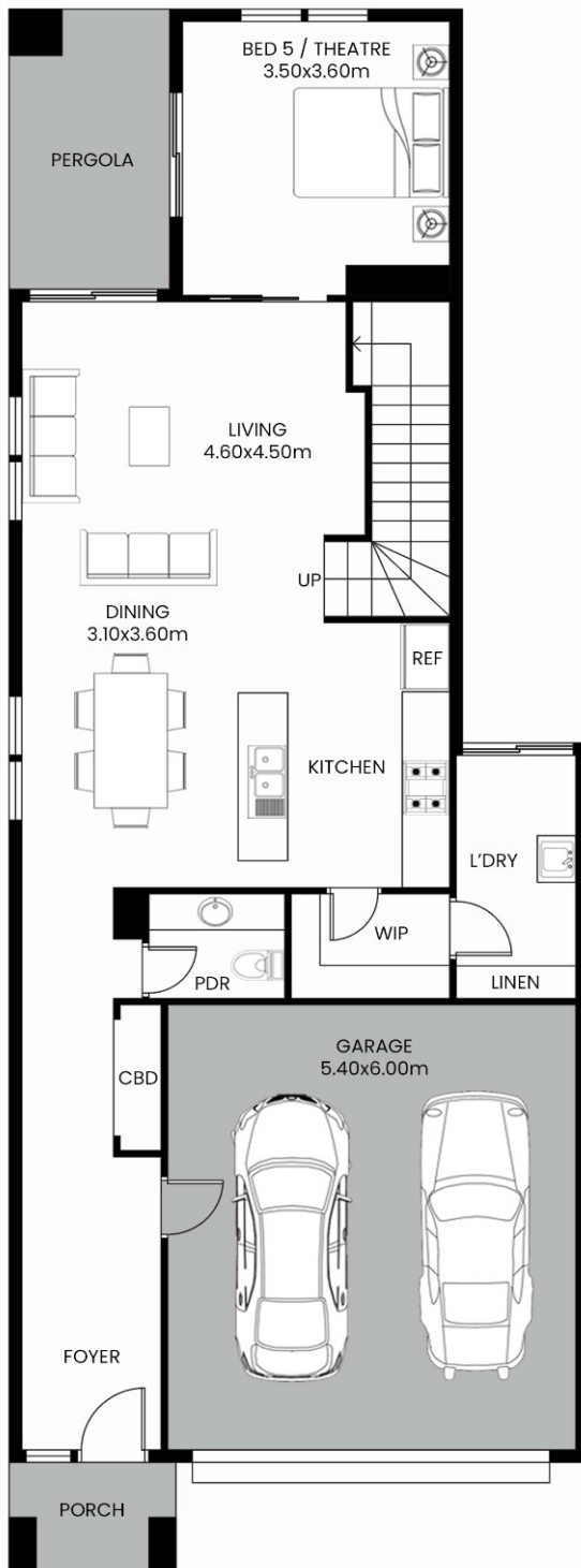
GROUND FLOOR
