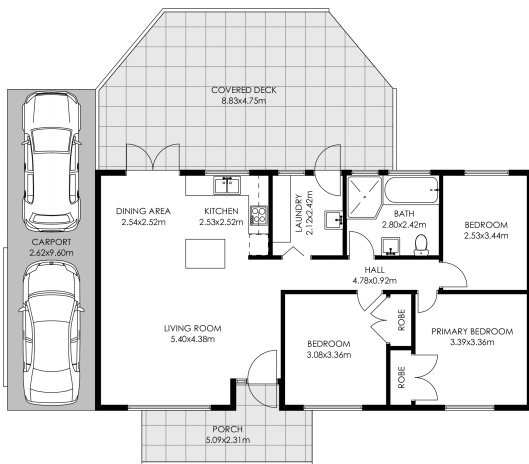
FLOOR PLAN
