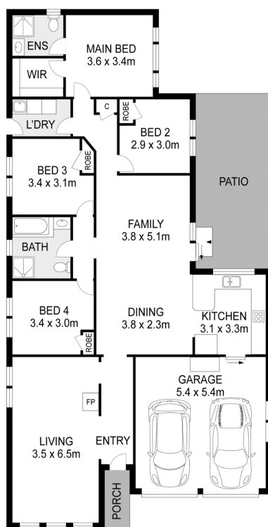
FLOOR PLAN
