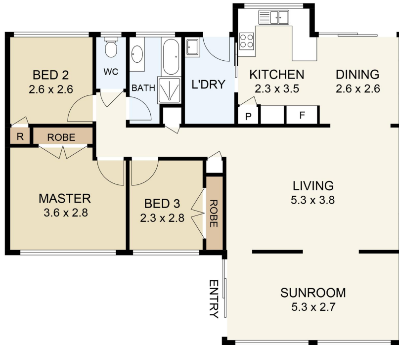
Floor Plan
