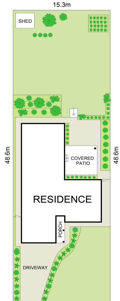
SITE PLAN
