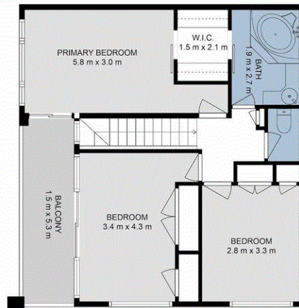
FLOOR 2
