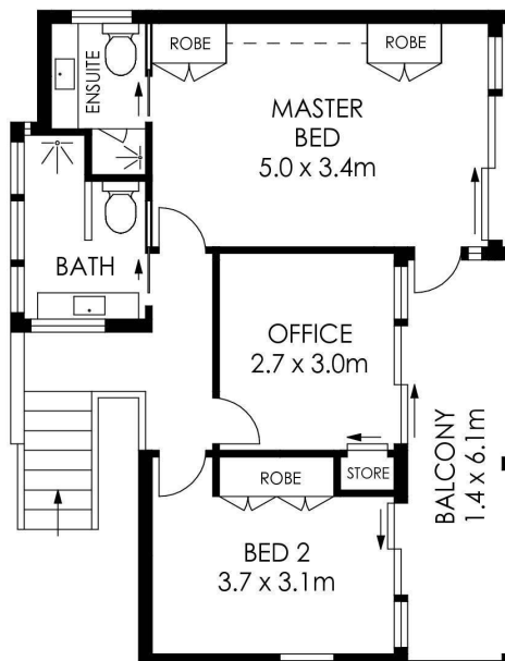
UPPER LEVEL
