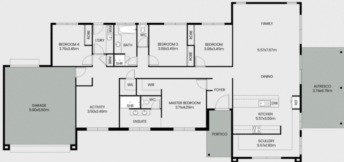
FLOOR PLAN
