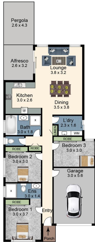
Floor Plan
