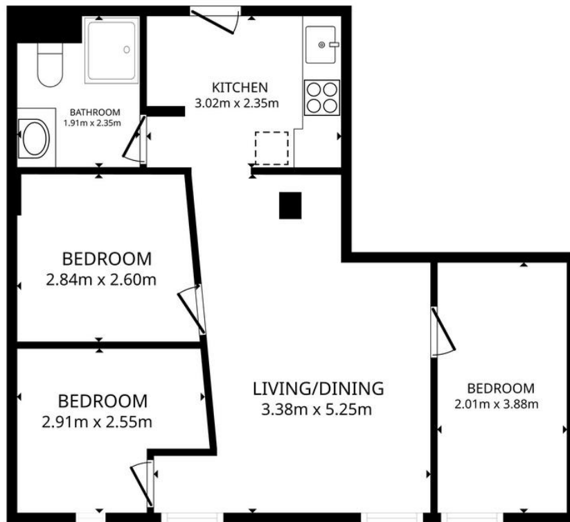
FLOOR PLAN
