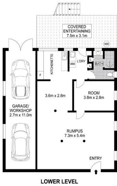
LOWER LEVEL
